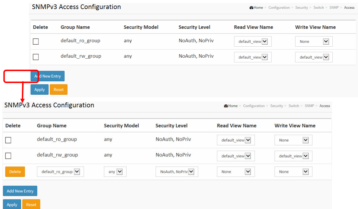
Figure 2-5.1.7.7: The SNMP Accesses Configuration
