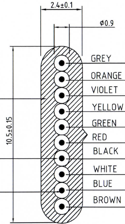
SECTION K-K
